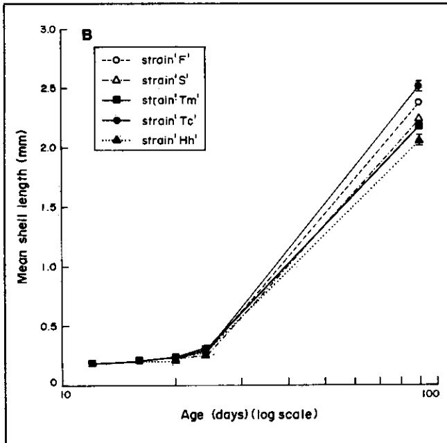
Fig. 2. Growth of T. gigas larvae/juveniles given zooxanthellae from various sources: fast (F) and slow (S) growers of a cohort of T. gigas , T. crocea (Tc), T. maxima (Tm), and Hippopus hippopus (Hh). Confidence limits at P < 0.05 level are shown. 2a shows the first phase, up to 24 days, and 2b shows both phases up to 90 days.
