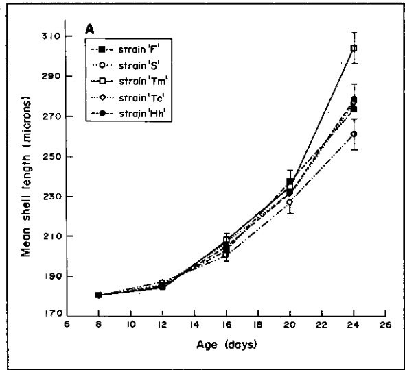
Fig. 2. Growth of T. gigas larvae/juveniles given zooxanthellae from various sources: fast (F) and slow (S) growers of a cohort of T. gigas , T. crocea (Tc), T. maxima (Tm), and Hippopus hippopus (Hh). Confidence limits at P < 0.05 level are shown. 2a shows the first phase, up to 24 days, and 2b shows both phases up to 90 days.
