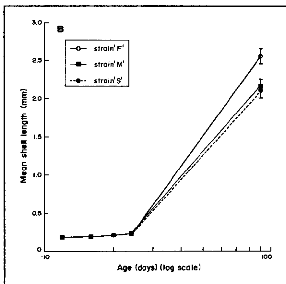
Fig. 1. Growth of T. gigas larvae/juveniles given zooxanthellae from fast (F), medium (M) and slow (S) growers of a cohort of T. gigas . Confidence limits at P < 0.05 level are indicated. 1a shows the growth in the first phase, up to day 24, and 1b shows both phases of growth, up to 90 days.
