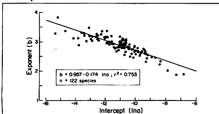
Fig. 1. Scatter plot, linear regression equation and coefficient of determination ( r^2 ) for the relationship between b and \ln a , based on data from Torres (1991).
