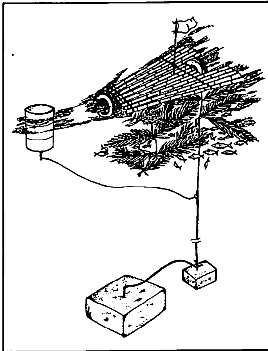
Fig. 4. The payao , a raft made of bamboo lashed together in a V-shape, is used to attract pelagic fishes. 40
