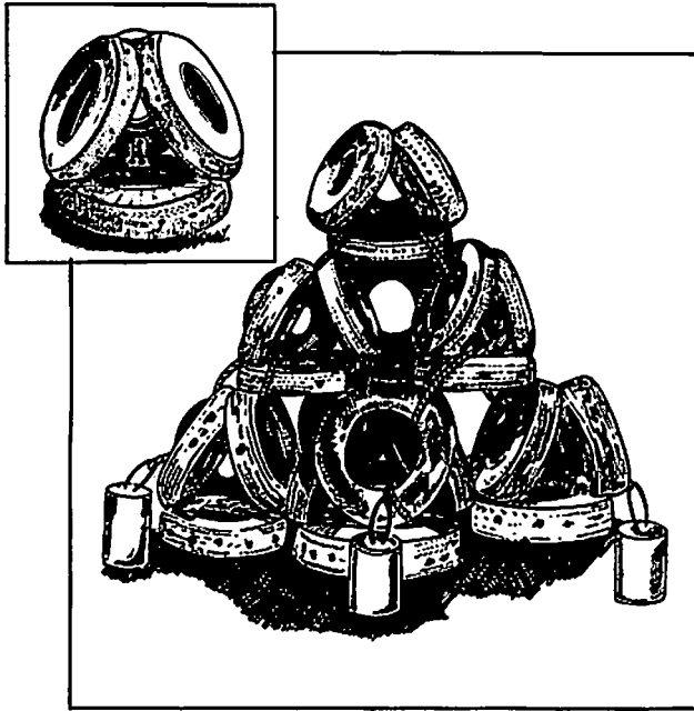
Fig. 5. Tire module of 36 tires anchored with four weights. 34
