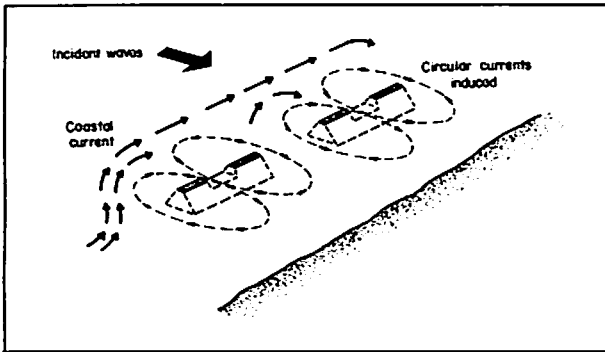
Fig. 17. Creation of circular currents with submerged breakwaters to enhance recruitment of abalone larvae. 60
