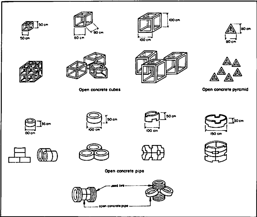
Fig. 10. Various modules of open concrete cubes, pipes and pyramids used in Thailand. 50
