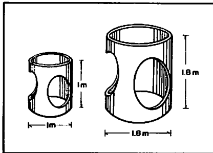
Fig. 9. Small and large reef units used off Hokkaido, Japan, to enhance habitat for octopus. 49
