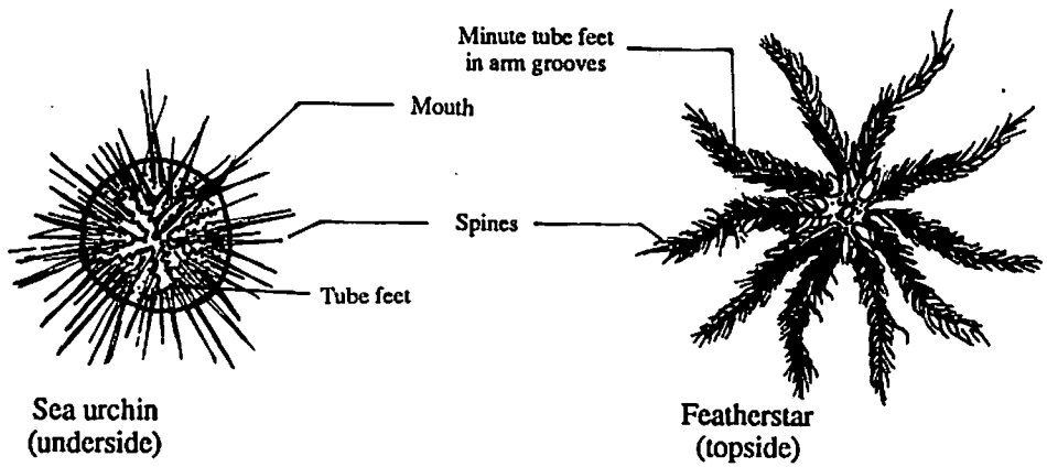
Fig. 11. Common echinoderms.
