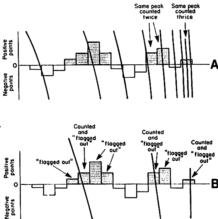
Fig. 2. Schematic representation, for a given "restructured" length-frequency sample of length classes counted and/or "flagged out" in computation of ESP (solid lines represent hypothetical growth curves).
