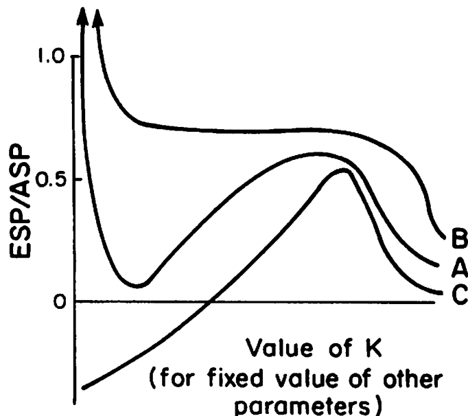
Fig. 1. Schematic representation of three types of response (= ESP/ASP values) obtained for given values of K, fixed values of the other parameters ( L_{\infty} , C, WP) and a given set of length-frequency data.
