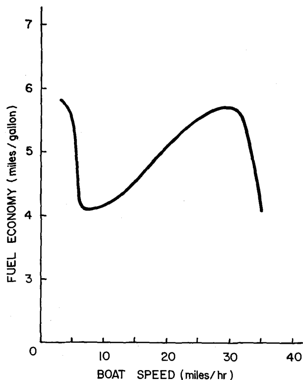
Fig. 3. Fuel consumption curve for an outboard with high horsepower.
