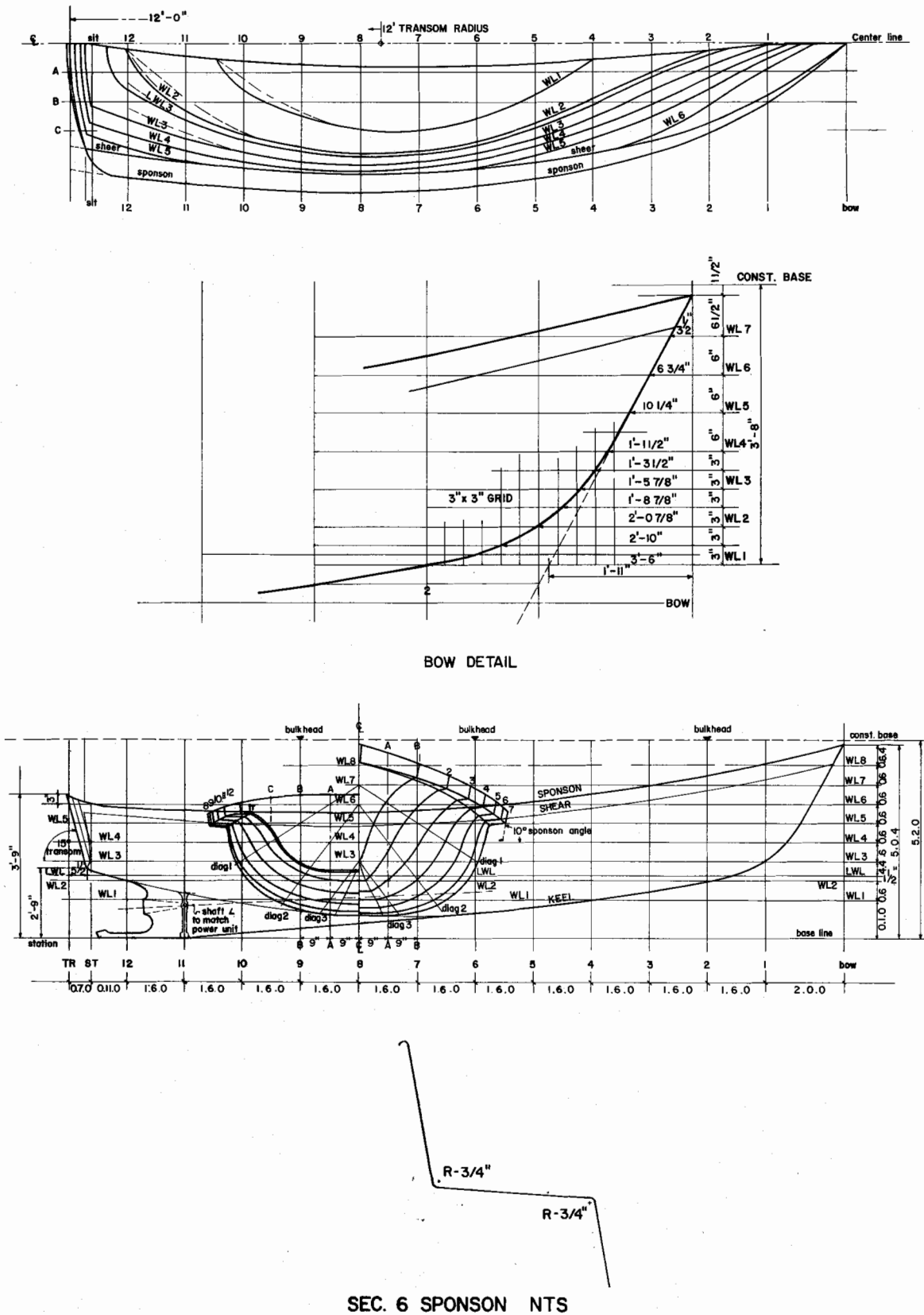
Fig. 1. Design plans for 1/12-scale model of 20-ft ICLARM prototype boat.
