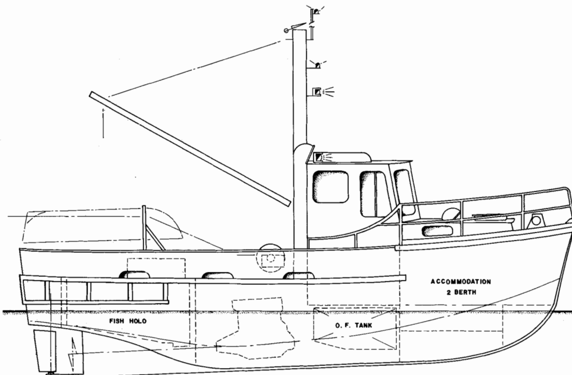
Fig. 4. A 27-ft general purpose vessel suitable for shrimp trawling and gillnetting.
