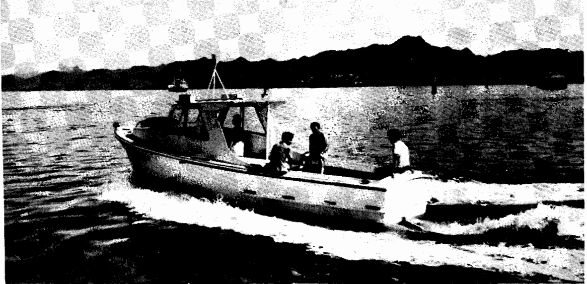
Fig. 7. Boat built from Fig. 3 design, running at 12 knots at design trim.
