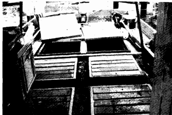
Fig. 5. View of Sandra Ann 's deck space looking aft from door of the house. The four live wells are shown in the foreground with the slatted voers in place. The main fish hold (hatch covers removed) is behind the live wells. Box with the stove is at left. Note the long unobstructed working space extending aft.
