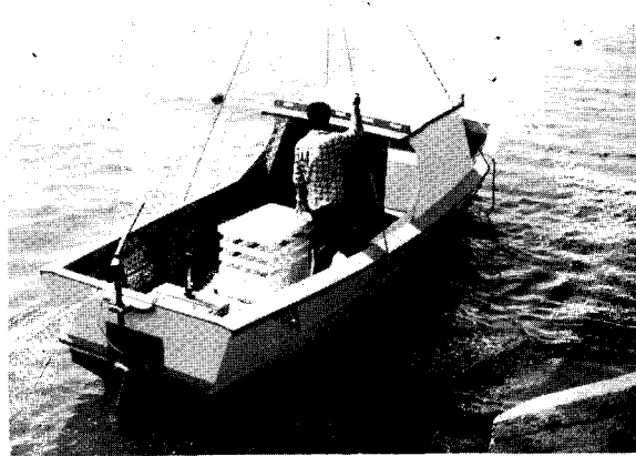
Fig. 1. Type A boat: a 28-ft, single-hull, diesel boat with removable propeller for shallow draft.
