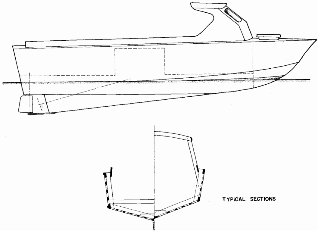
Fig. 1. Typical layout for a modified 27-ft stock hull.
