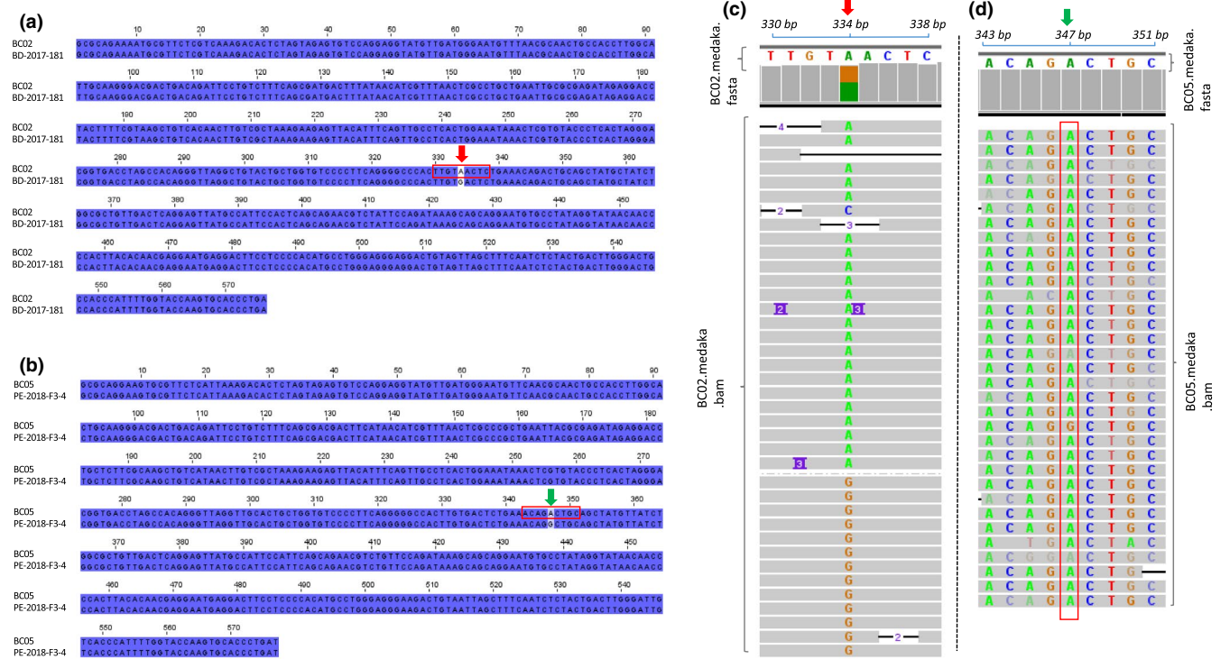
FIGURE 2 (a and b) Identification of single nucleotide polymorphisms (SNPs) using sequences alignment of TiLV segment 1 medaka consensus sequences (this study) with their closest Sanger verified references. (a) Bangladeshi BC02 consensus (576 bp) aligned with BD-2017-181 (MT466437.1) showing SNP in position 334 (red arrow); (b) Peruvian BC05 consensus (577 bp) aligned with PE-2018-F3-4 (MK425010.1) with SNP in position 347 (green arrow); (c and d) SNPs examination in Integrative Genomics Viewer (IGV) (version 2.8.10); (c) Read depth (BC02.medaka.bam file) aligned with final medaka consensus sequence (BC02.medaka.fasta file) showing the SNP is partitioned between 274 and 620 bp amplicons; (d) Read depth (BC05.medaka.bam file) aligned with final medaka consensus sequence (BC05.medaka.fasta file) confirming the SNP is real since it is identical in 97% of the reads, except for 1 homopolymer base-call error: G
