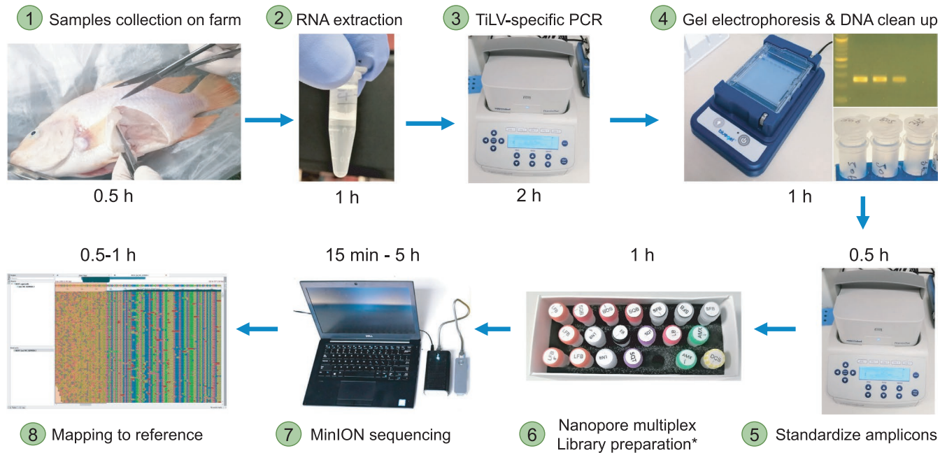
FIGURE 1 Overall workflow from sample collection of diseased fish on farm to sequence results. The entire process takes less than 12 hr. * DNA repair, end-preparation, multiplex native barcode and adapter ligation
