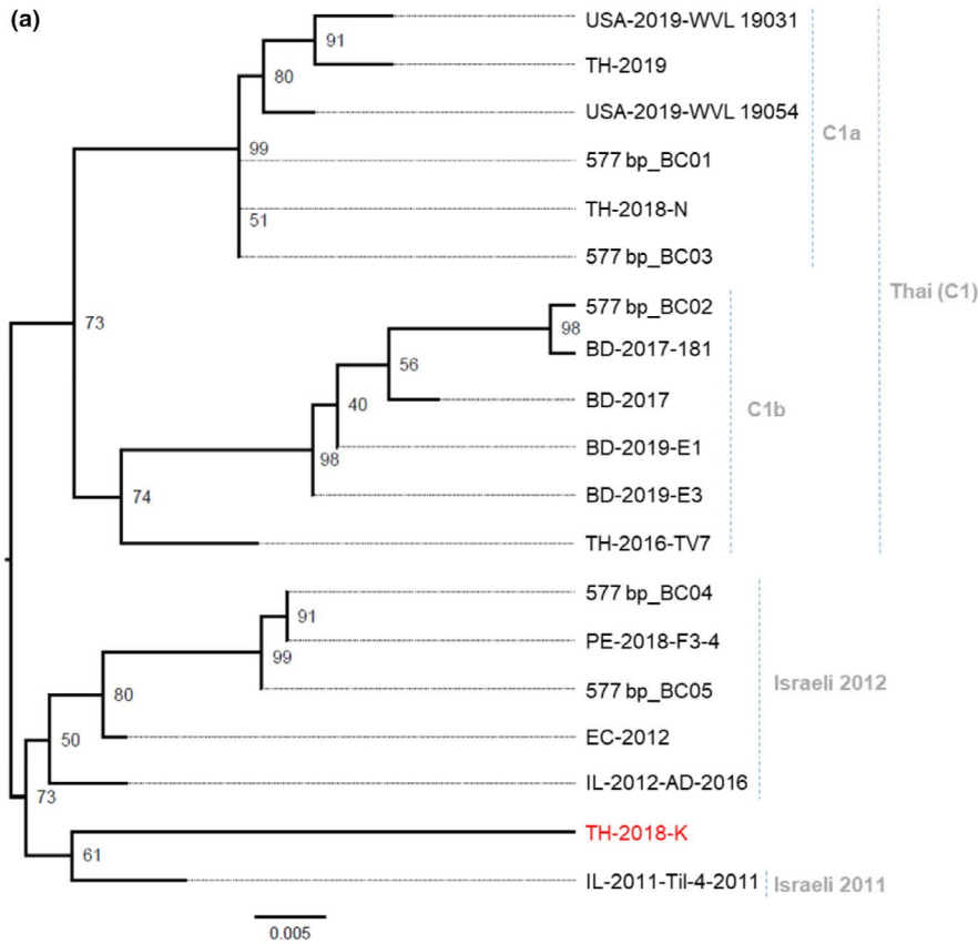
FIGURE 3 Maximum likelihood trees constructed in IQ-TREE based on the nucleotide consensus sequences alignment of short TiLV consensus (577 bp and 231 bp) with TiLV segment 1 reference sequences retrieved from GenBank database (Table 1). (a) Five 577 bp consensus sequences compared with 14 reference sequences trimmed to 577 bp. (b) five 577 bp consensus sequences trimmed to 231 bp, five original 231 bp consensus sequences compared with 14 reference sequences trimmed to 231 bp. The branch lengths indicate the number of substitutions per site, and node labels indicate bootstrap support values in percentage. Trees rooted using the mid-point rooting method
